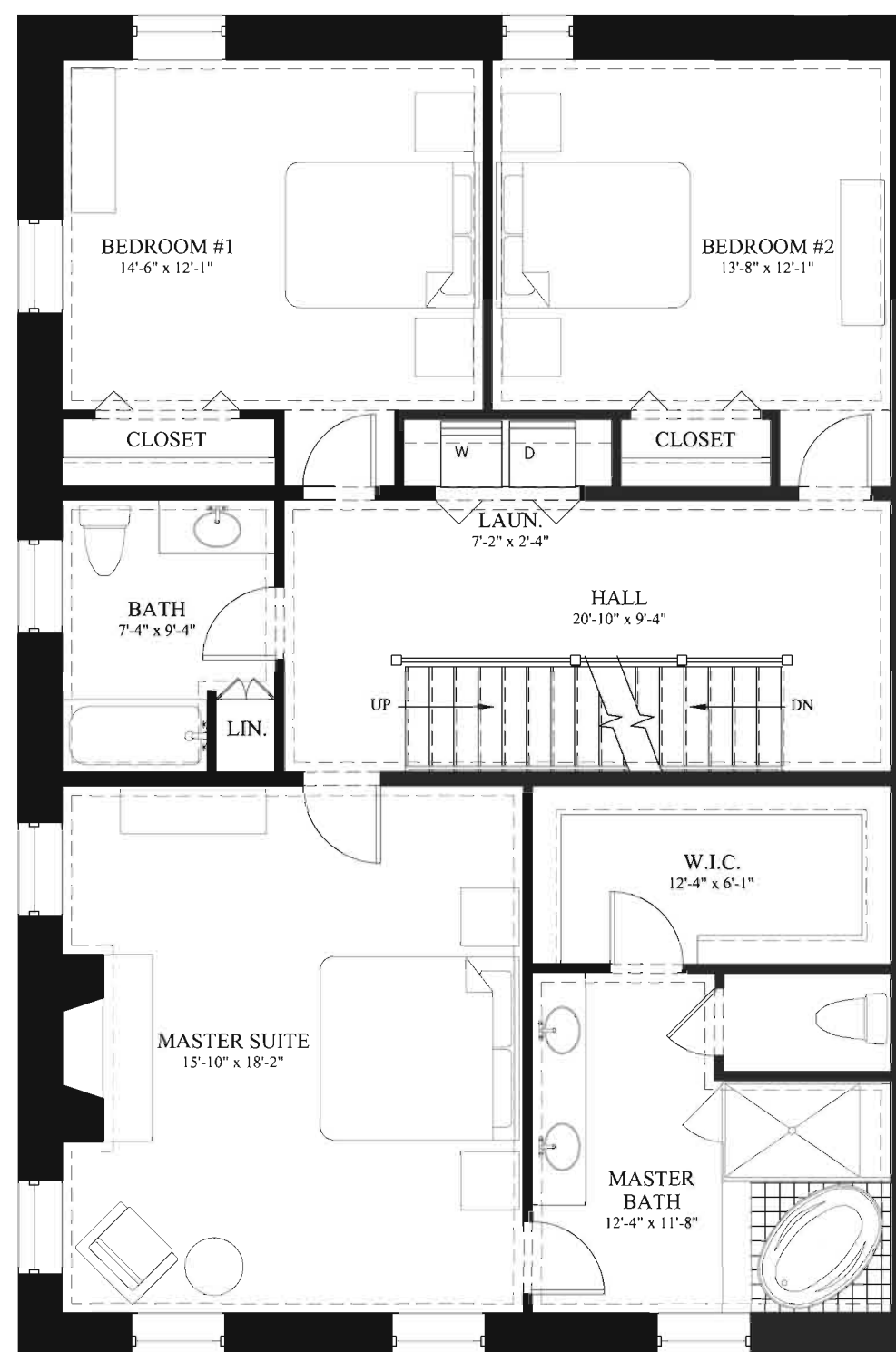
SECOND FLOOR - NORTH SCALE: 1/4" = 1'-0"
