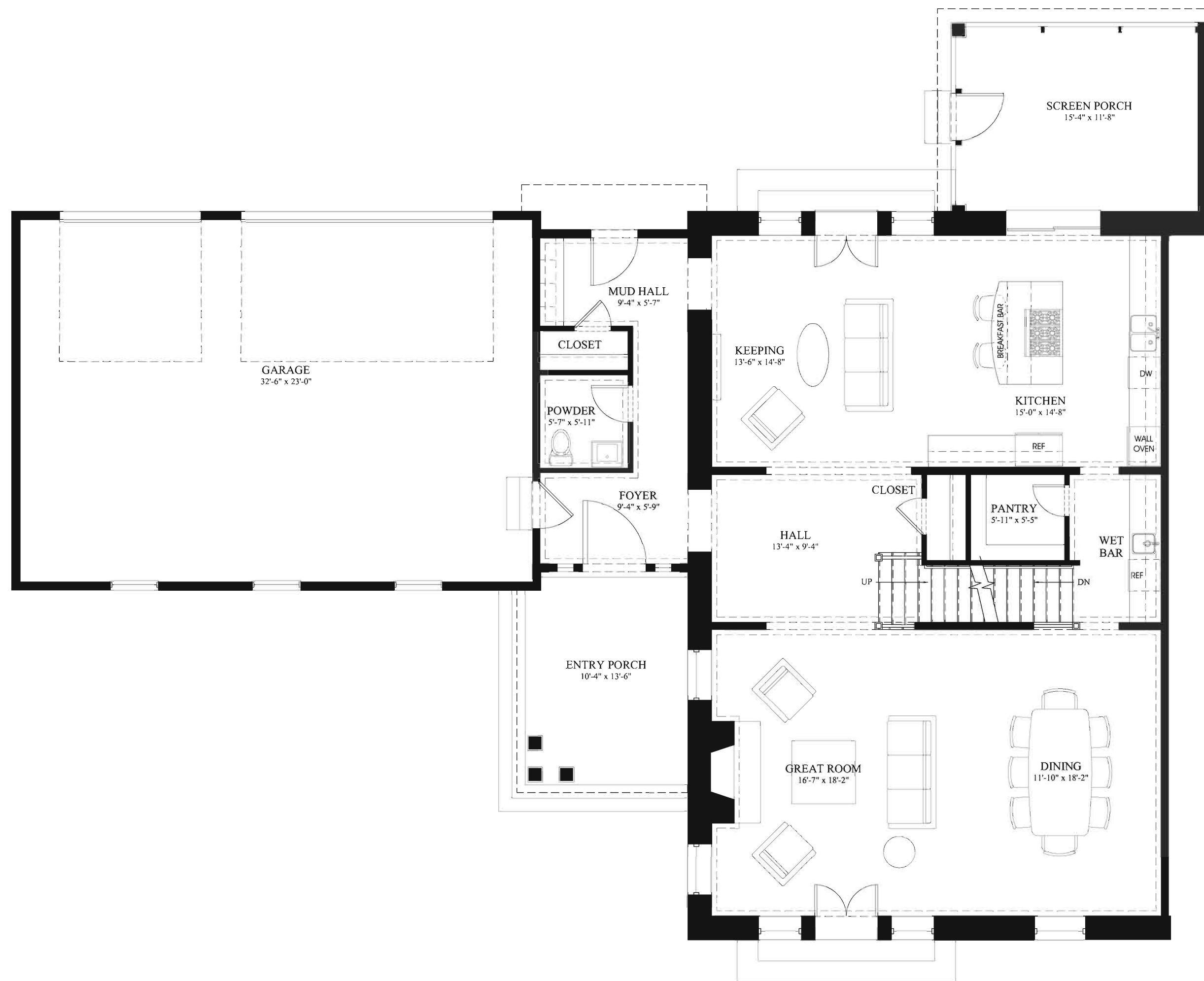
FIRST FLOOR - NORTH SCALE: 1/4" = 1'-0"
